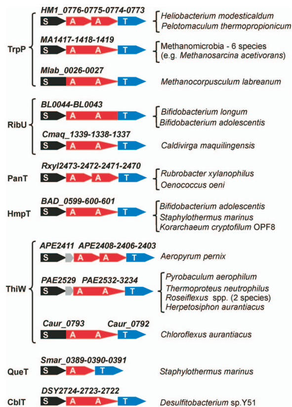
FIG. 2. Genomic organization of the group I ECF transporters containing S components from the TrpP, RibU, PanT, HmpT, ThiW, QueT, and CblT families. Genes encoding substrate capture S components and A and T components of the dedicated energy-coupling modules are shown by black, red, and blue arrows, respectively.
